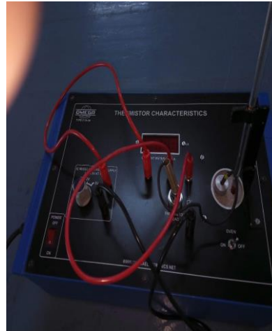
Thermistor Characteristics
